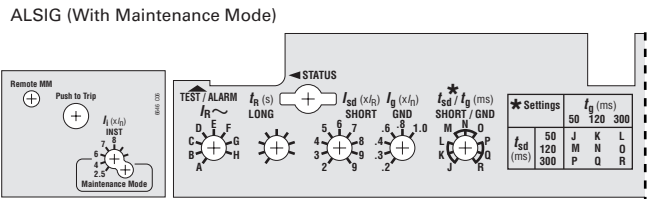
SD/ GF Delay Settings Table
