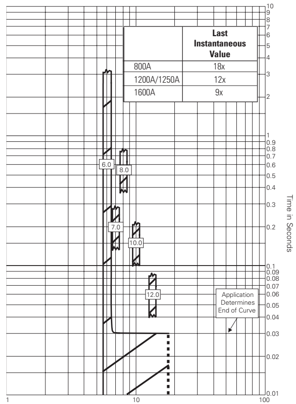
Instantaneous Mode Trip
