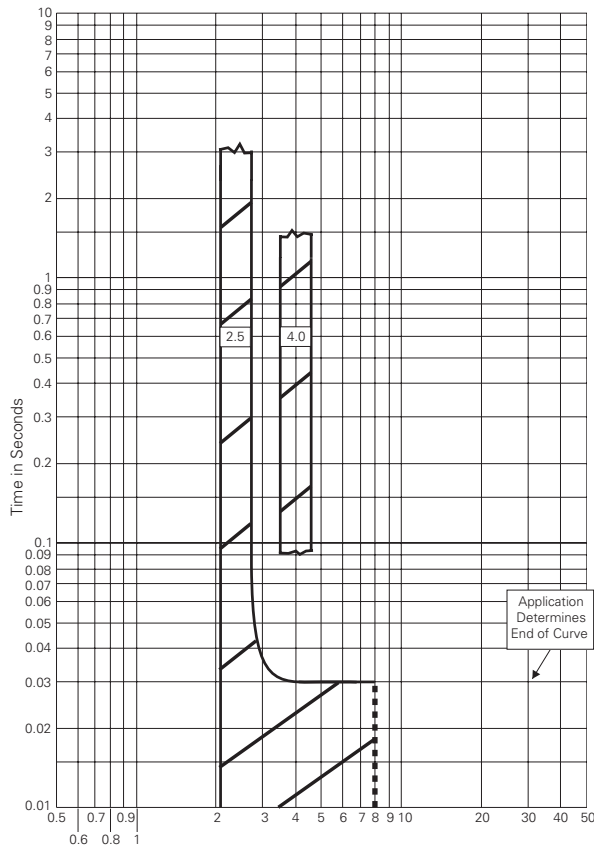
Maintenance Mode Trip
