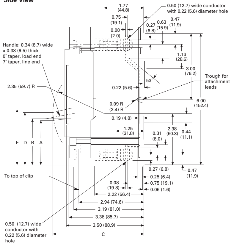
Side View
