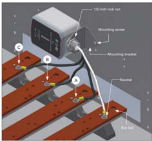
Surge suppression devices shown are field installed into Group Metering Main Breaker Devices. 1PMB and 3PMB series.
