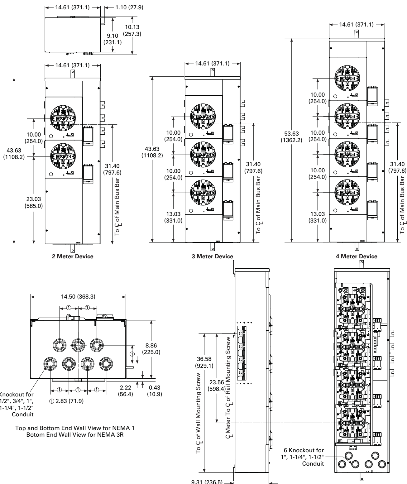
Lever Bypass 125 A Meter Module (3-phase IN 1-phase OUT NEMA 3R shown)
