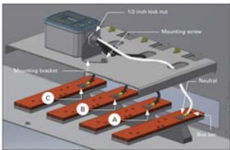
Surge suppression devices shown are field installed into Group Metering Main Breaker Devices. 1PMB and 3PMB series.
