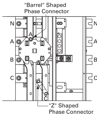
FACTORY 200 A A-B PHASING
