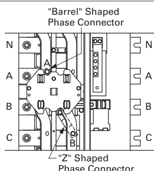
FACTORY 125 A A-B PHASING
