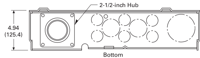
Bottom MBE4040B200BSH
