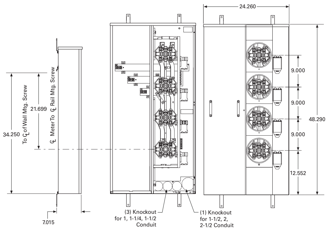
3, 4 Meter Device
