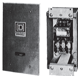
Flush Mounting Starter Pullbox and Mounting Strap with Plaster Adjustment Feature
