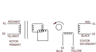
SCHEMATIC DRAWING FOR BRUSHLESS RESOLVER
