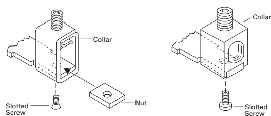
T250KB Terminal
