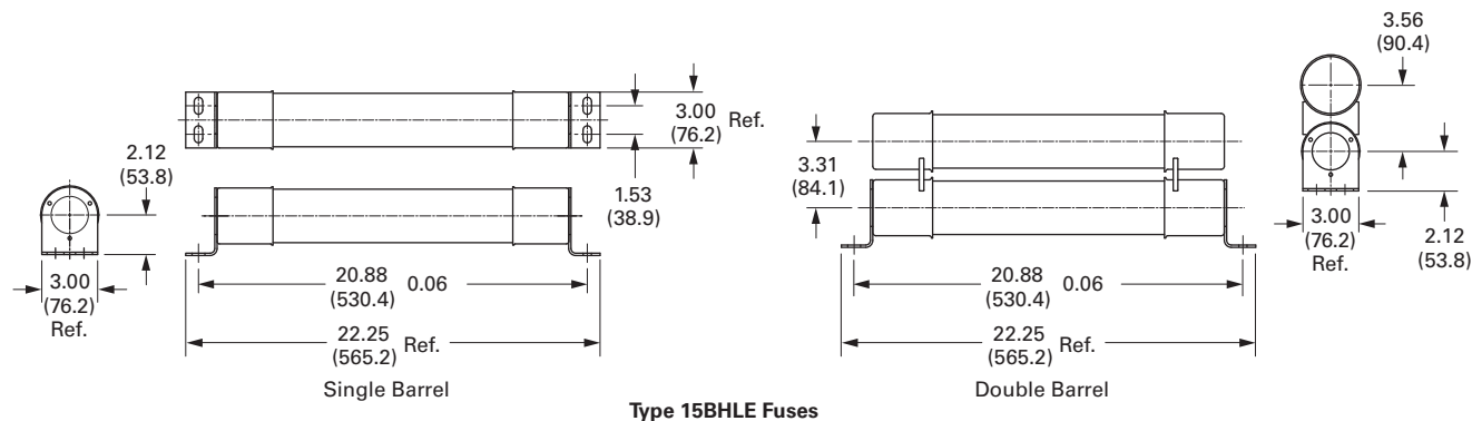
Type 15BHLE Fuses
