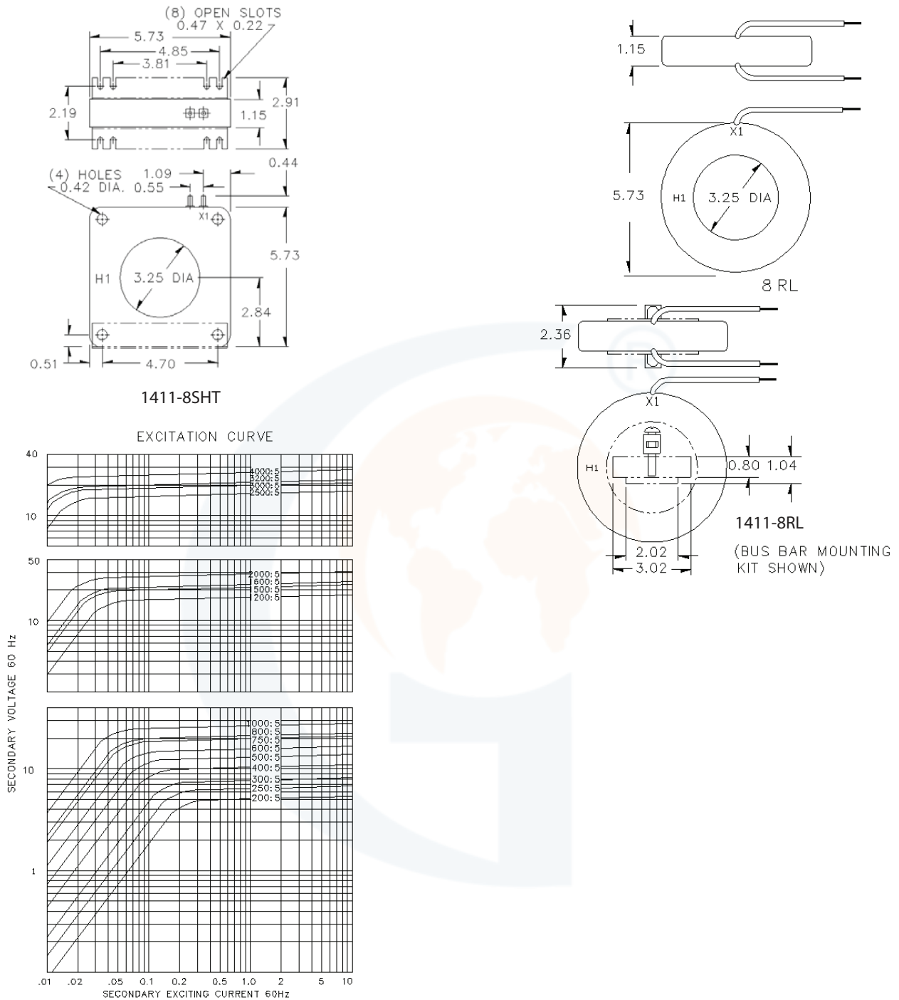
Figure 2 - 1411-8xxx Dimensions
