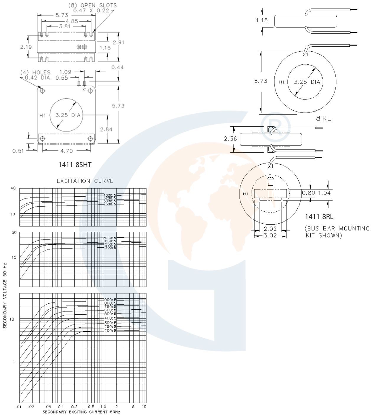
Figure 2 - 1411-8xxx Dimensions
